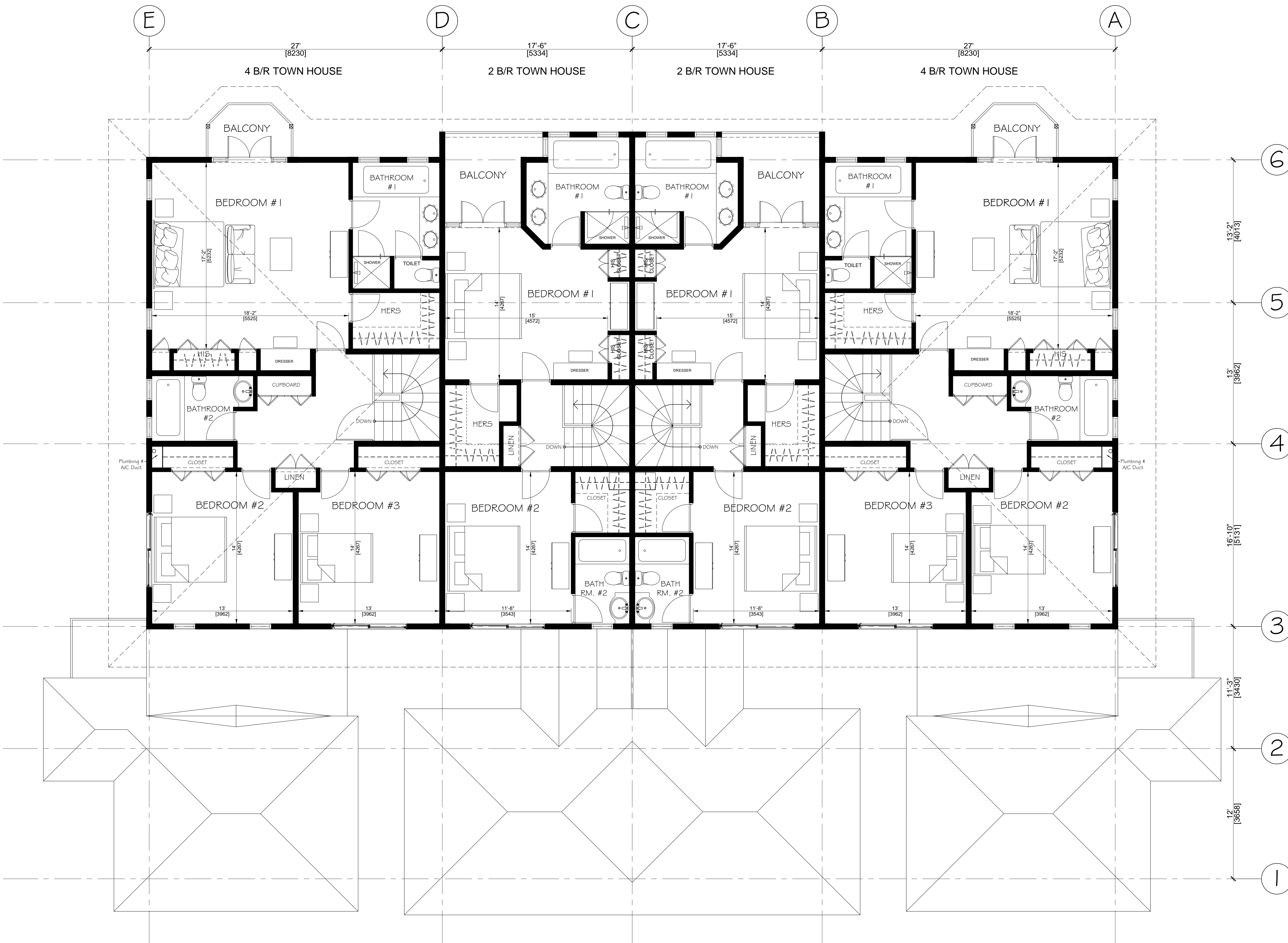
UPPER FLOOR PLAN SCALE 1/4" = 1'-0"
